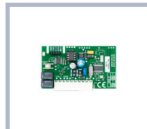
ONE.2WI 433.92 MHz receiver with power supply 12±28 VDC / 21±28 VAC, 2 channels with triple coding: Advanced Rolling Code and Rolling Code, plug-in. 512 memorisable codes.
